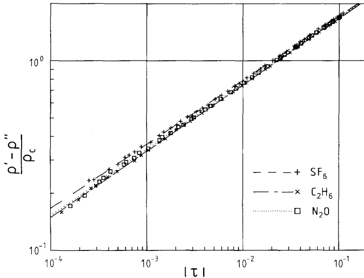
Fig. 5. Reduced density difference between coexisting liquid and vapor versus reduced temperature difference for \text{SF}_6 , \text{C}_2\text{H}_6 , and \text{N}_2\text{O} .
