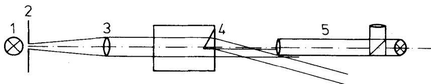
Fig. 3. Schematic diagram of refractometer: 1, Hg-spectral lamp; 2, slit; 3, lens; 4, prism; 5, autocollimating telescope.
