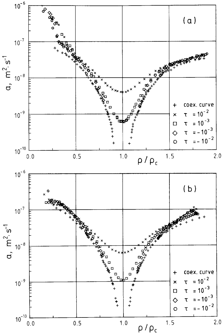
Fig. 7. Thermal diffusivity versus reduced density for SF 6 (a), C 2 H 6 (b), and N 2 O (c).
