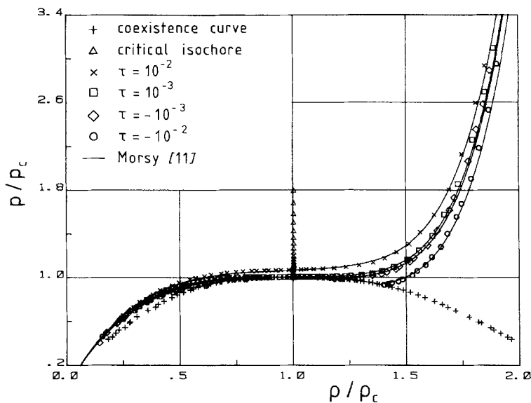
Fig. 6. Reduced pressure versus reduced density for SF 6 .
