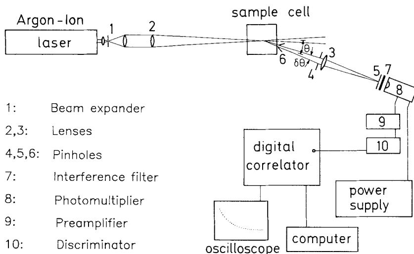
Fig. 2. Schematic diagram of dynamic light-scattering apparatus.
