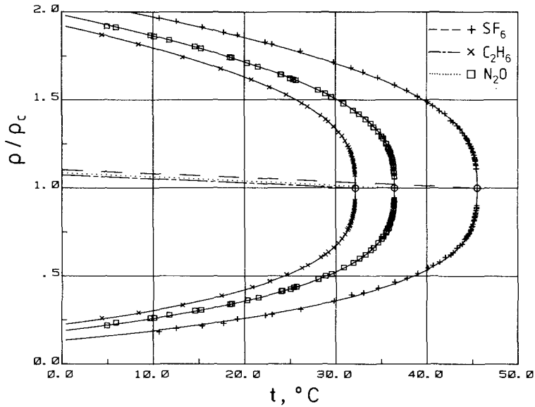
Fig. 4. Reduced density versus temperature for coexisting liquid and vapor for SF 6 , C 2 H 6 , and N 2 O.
